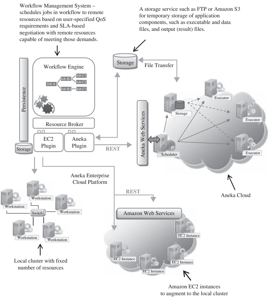
FIGURE 12.1. Workflow engine in the cloud.
